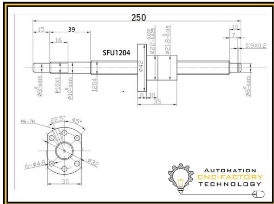
Vite asse Z DT-3T a ricircolo di sfere, ROLLED BALLSCREW SFU1204-C7-DIN69051
